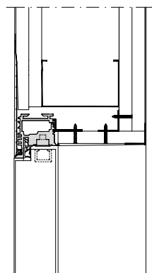
Verticale doorsnede reverse openend in de deuropening (type RI)
